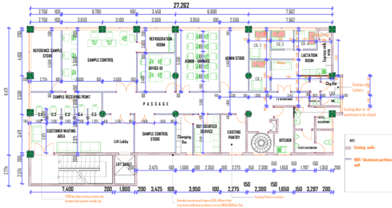
FIRST FLOOR LAYOUT PLAN - PHASE -1
